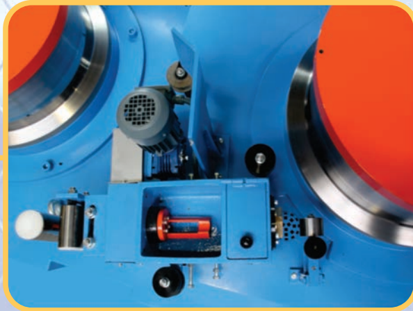
LUBRICANT MIXER
